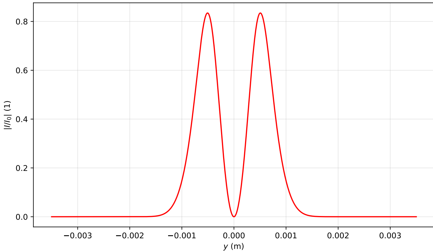
Intensity profile I(x=0, y, z=0.398)/I_0 , P_{in}=2.0P_{cr} , artificial time
